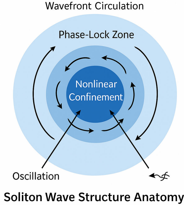
Figure 136: Soliton Wave Structure Anatomy. Schematic of the internal structure of a soliton in the ultronic medium. Phase-locked circulating wavefronts maintain stability, with nonlinear strain confinement preventing dispersion. This structure underlies the emergence of mass, spin, and charge from mechanical wave behavior in the UMH framework.
