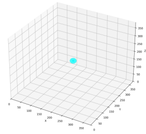
UMH Wave Propagation Speed 3D Wavefront Isosurface Step: 56
