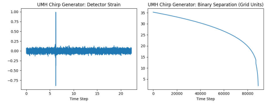
UMH Chirp Dynamic Preview - Livingston
