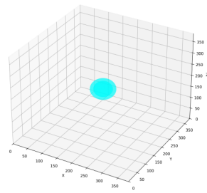
UMH Wave Propagation Speed 3D Wavefront Isosurface Step: 198
