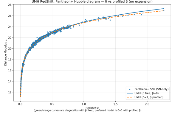
Figure 86: \delta vs. profiled \beta (diagnostic). Comparison of the diagnostic case with \delta free, \beta = 0 (solid) and the preferred case \delta = 1 with \beta profiled (dashed). The preferred curve tracks the data at high z .
