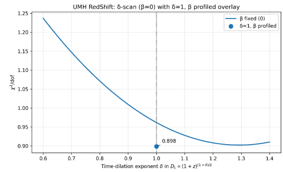
Figure 90: \chi^2/\text{dof} vs. \delta (diagnostic). With \beta fixed to 0 (solid), the minimum lies near \delta \approx 1.30 . The preferred point ( \delta = 1 , \beta profiled; dot) sits in the same trough with \chi^2/\text{dof} \approx 0.898 .
