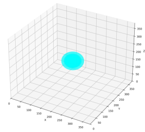
UMH Wave Propagation Speed 3D Wavefront Isosurface Step: 255
