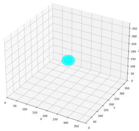
UMH Wave Propagation Speed 3D Wavefront Isosurface Step: 141
