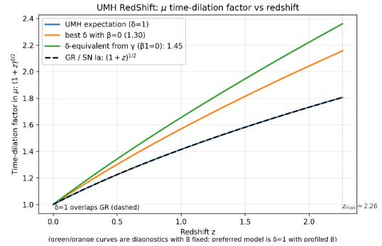
Figure 138: Time-dilation factor in the Hubble prediction. In the UMH expression \mu(z) = 5 \log_{10}(d(1 + z)^{(1+\delta)/2}/\sqrt{T(z)}) + 25 , the (1 + z)^{(1+\delta)/2} term encodes time dilation. With \delta = 1 , the curve tracks the SN Ia reference; attenuation T(z) handles the remaining flux evolution.
