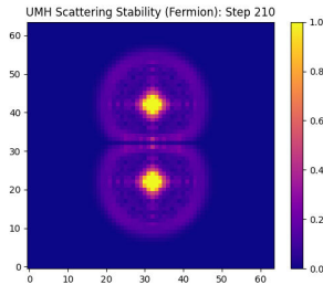
Fermionic solitons at step 210, showing separated anti-phased cores prior to interaction.
