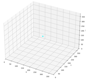
UMH Wave Propagation Speed 3D Wavefront Isosurface Step: 0
