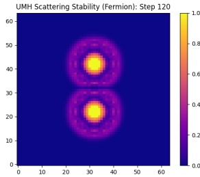
Fermionic solitons at step 120, showing separated anti-phased cores prior to interaction.
