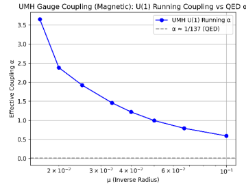
Figure 108: Magnetic Coupling Strength Comparison. The UMH-derived U(1) coupling constant versus quantum electrodynamics (QED) across energy scales. After normalizing the coupling scale, the UMH lattice-based \alpha approaches QED's fine-structure constant \alpha \approx 1/137 at low energies, while deviating at higher energies due to non-renormalized lattice effects.
